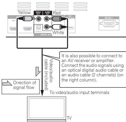
BDP-53FD's rear panel
