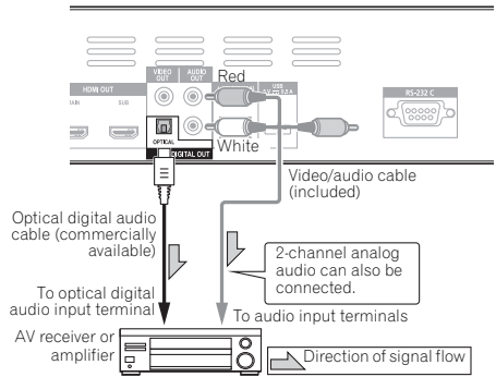
BDP-53FD's rear panel
